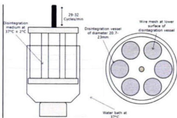
Disintegration apparatus
